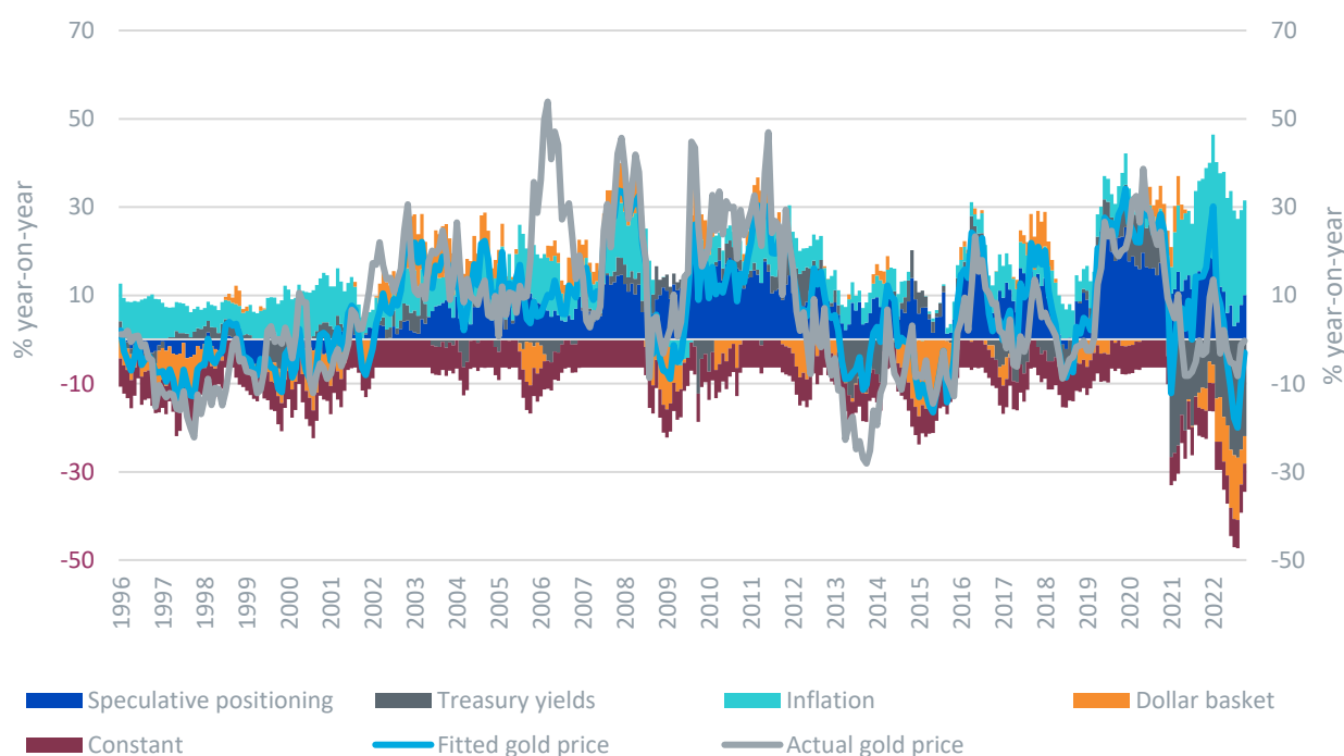
The impact of each variable: attribution of fitted results vs actual price
